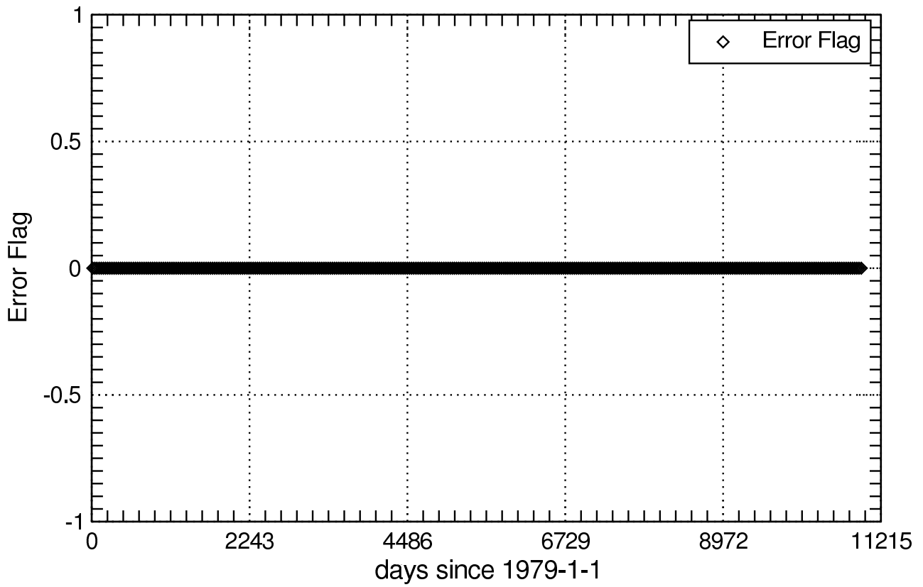
Error Flag of hcfc22global_Amon
