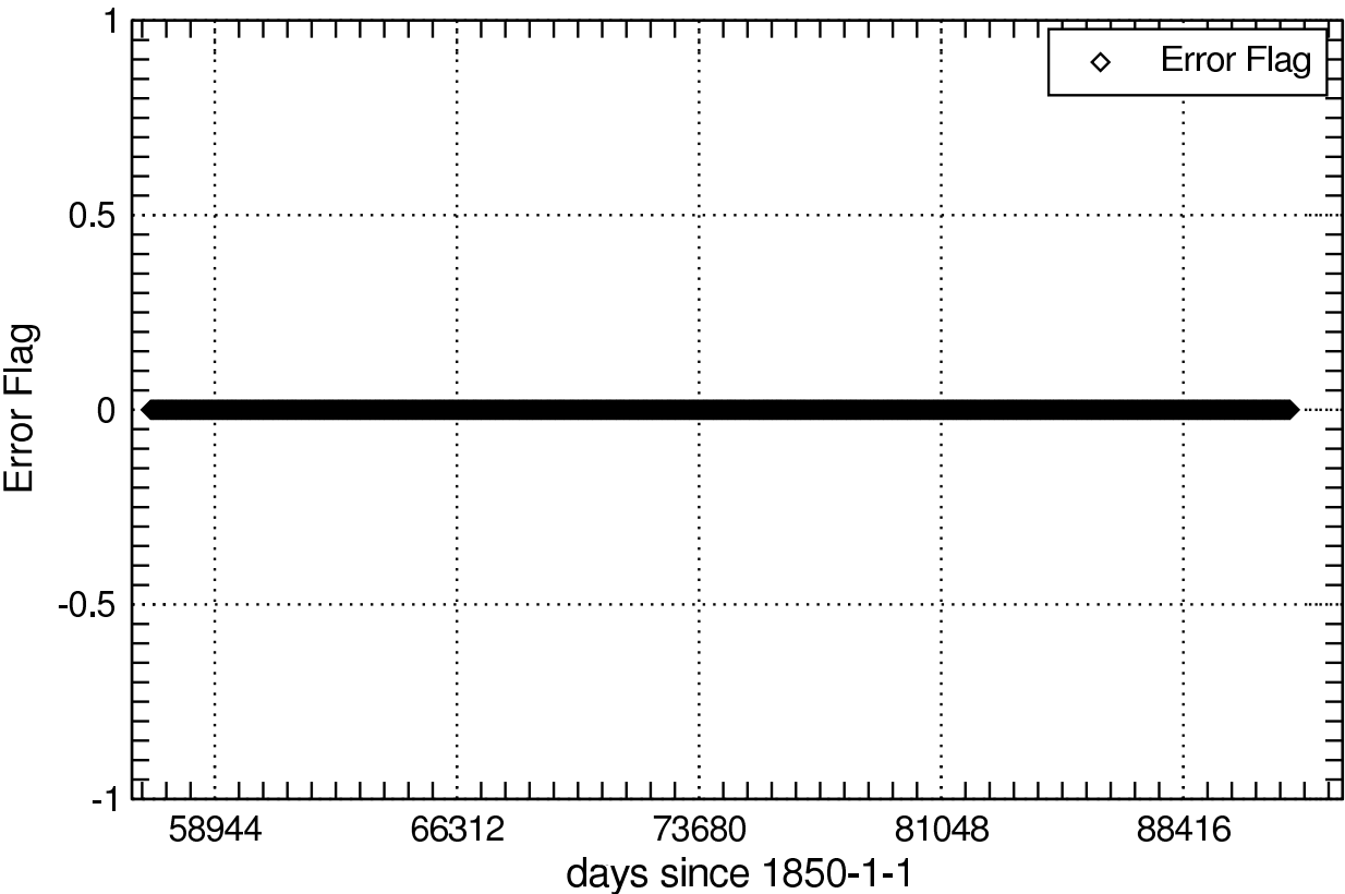
Error Flag of tasmax_Amon
