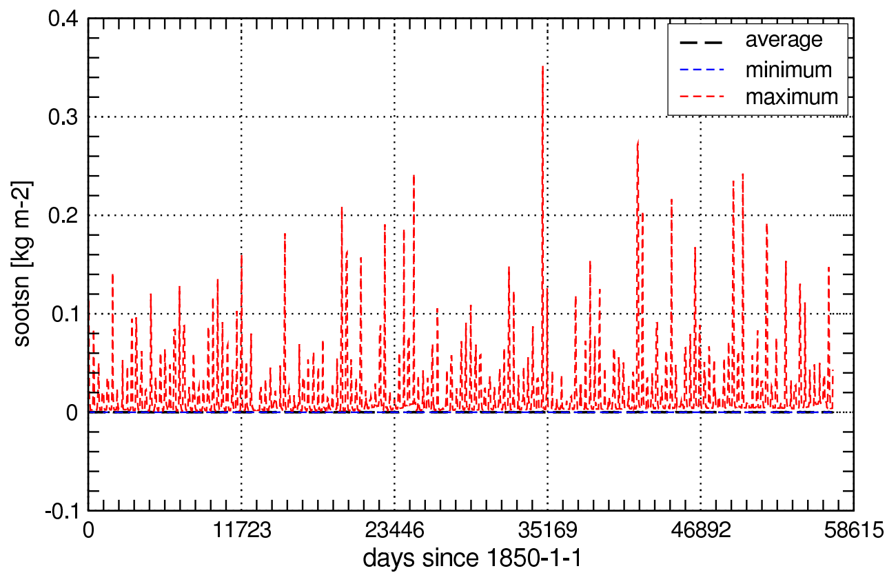
Global Values of sootsn_Llmon
