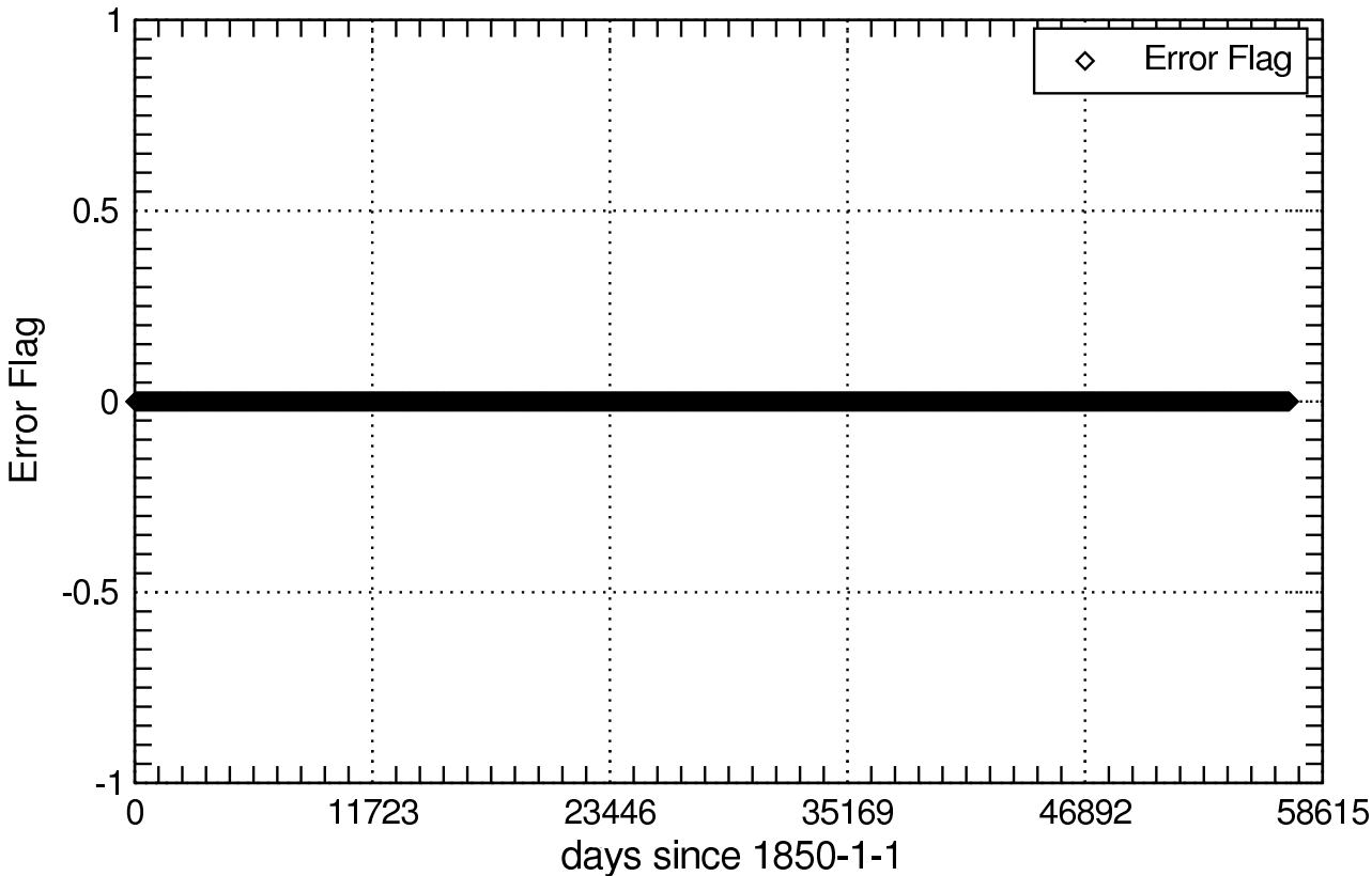
Error Flag of tran_Lmon
