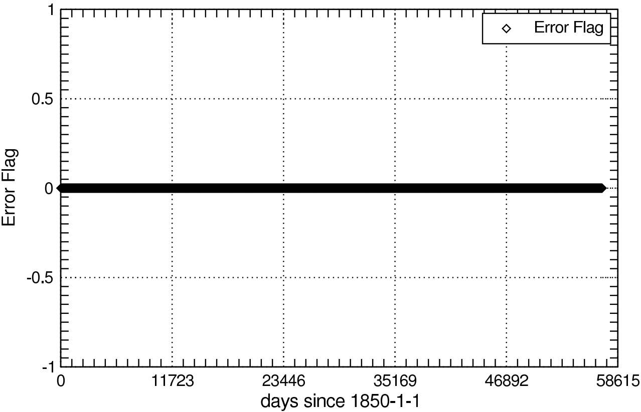
Error Flag of evpsblsoi_Lmon
