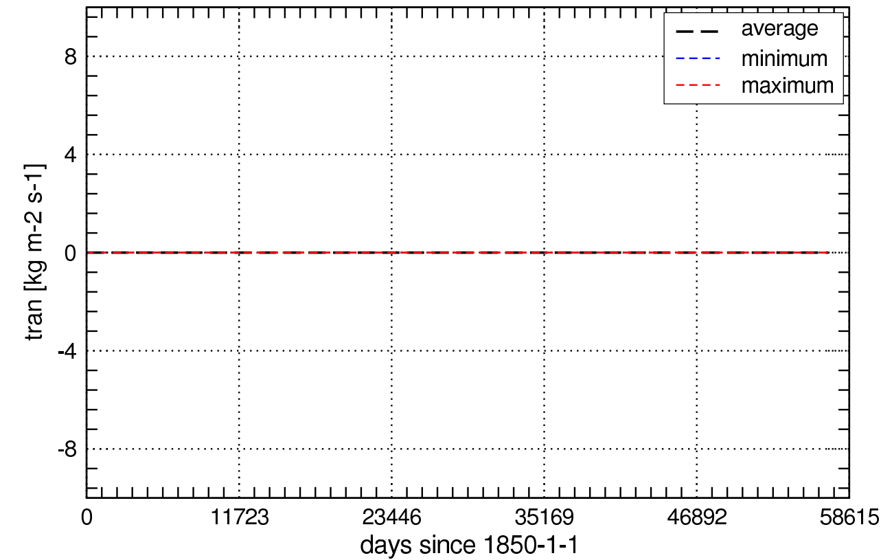
Global Values of tran_Lmon
