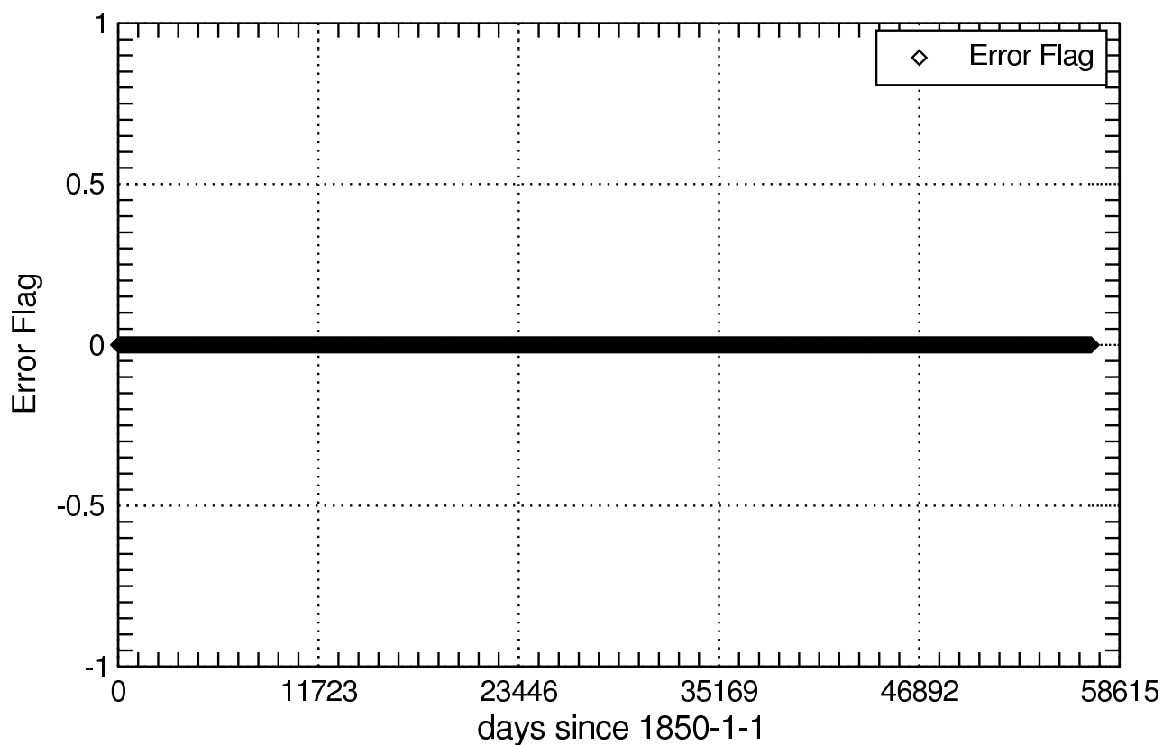
Error Flag of thetaoga_Omon
