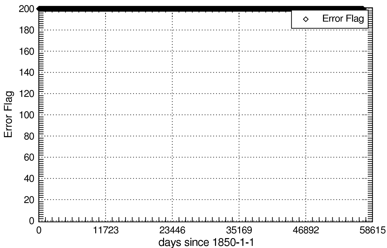
Error Flag of fco2antt_Amon
