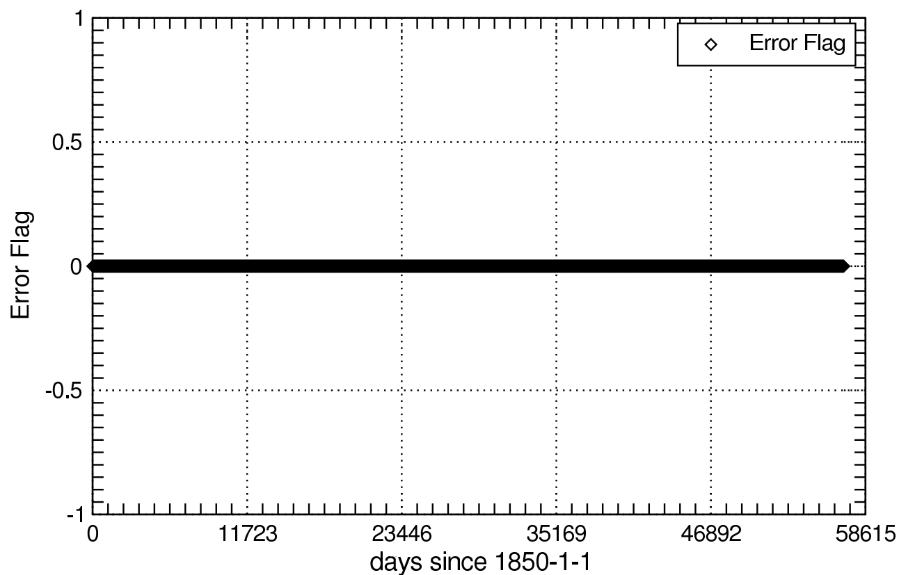
Error Flag of tasmax_Amon
