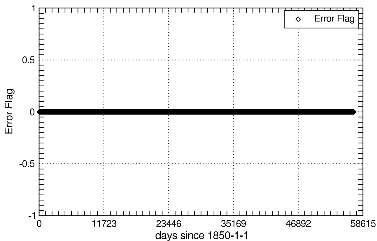
Error Flag of sootsn_Llmon
