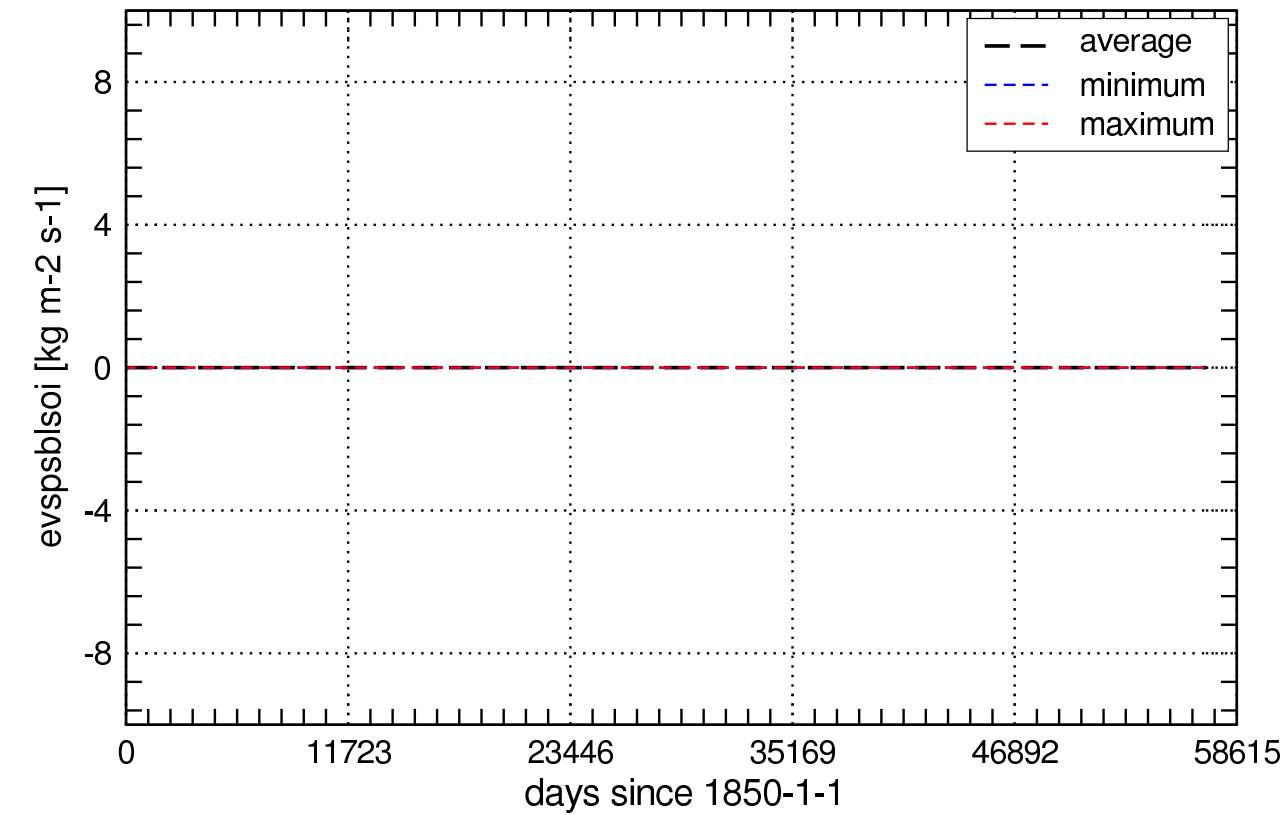
Global Values of evpsblsoi_Lmon
