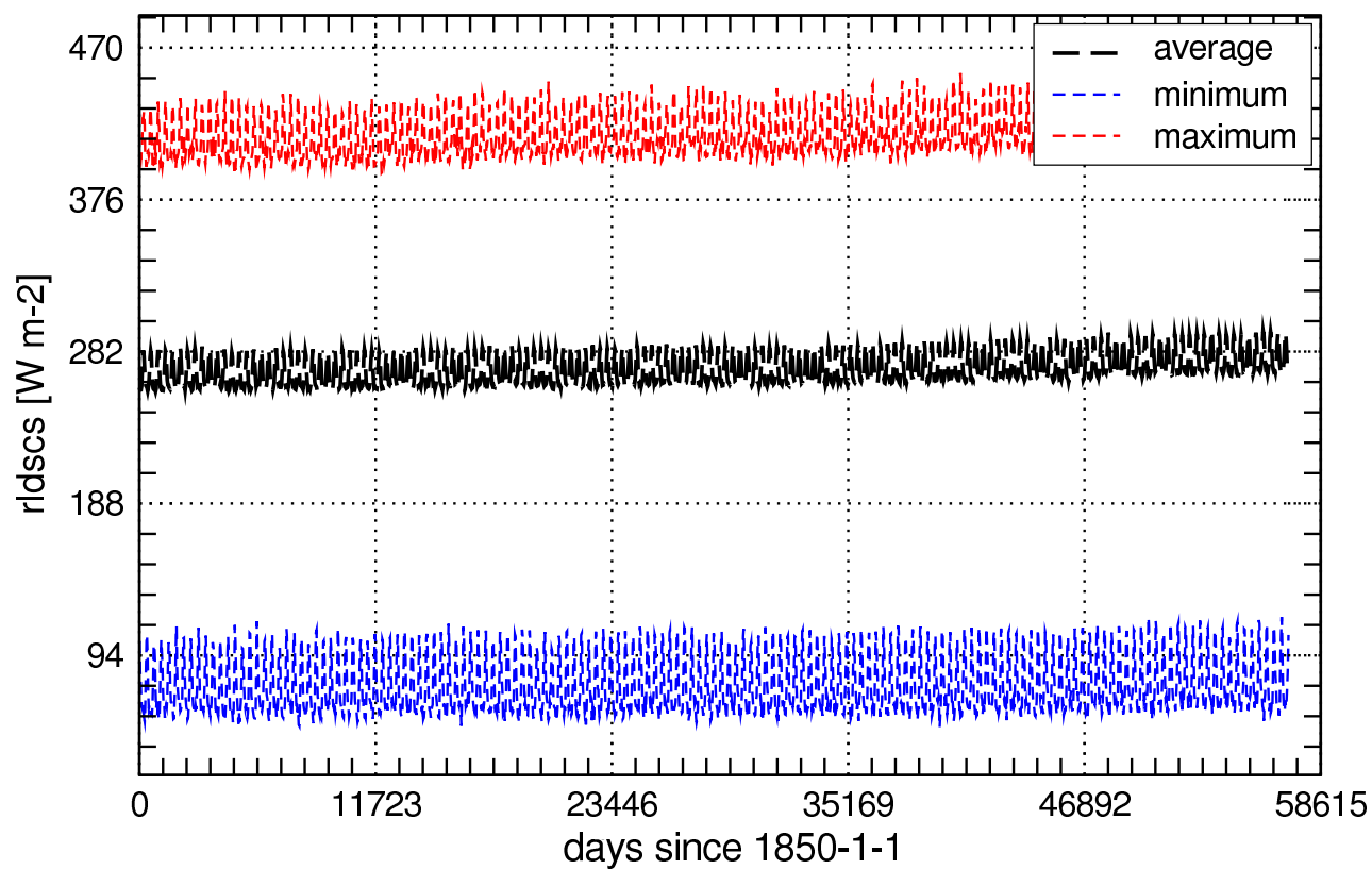
Global Values of rldscs_Amon
