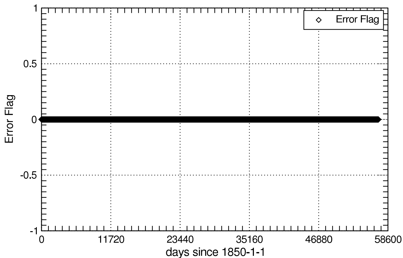
Error Flag of tossq_day
