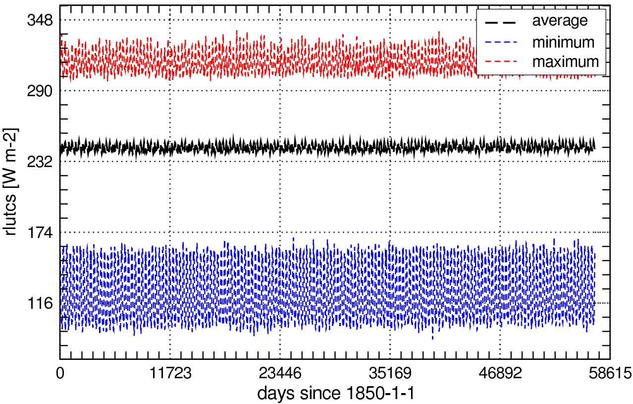
Global Values of rlutcs_Amon
