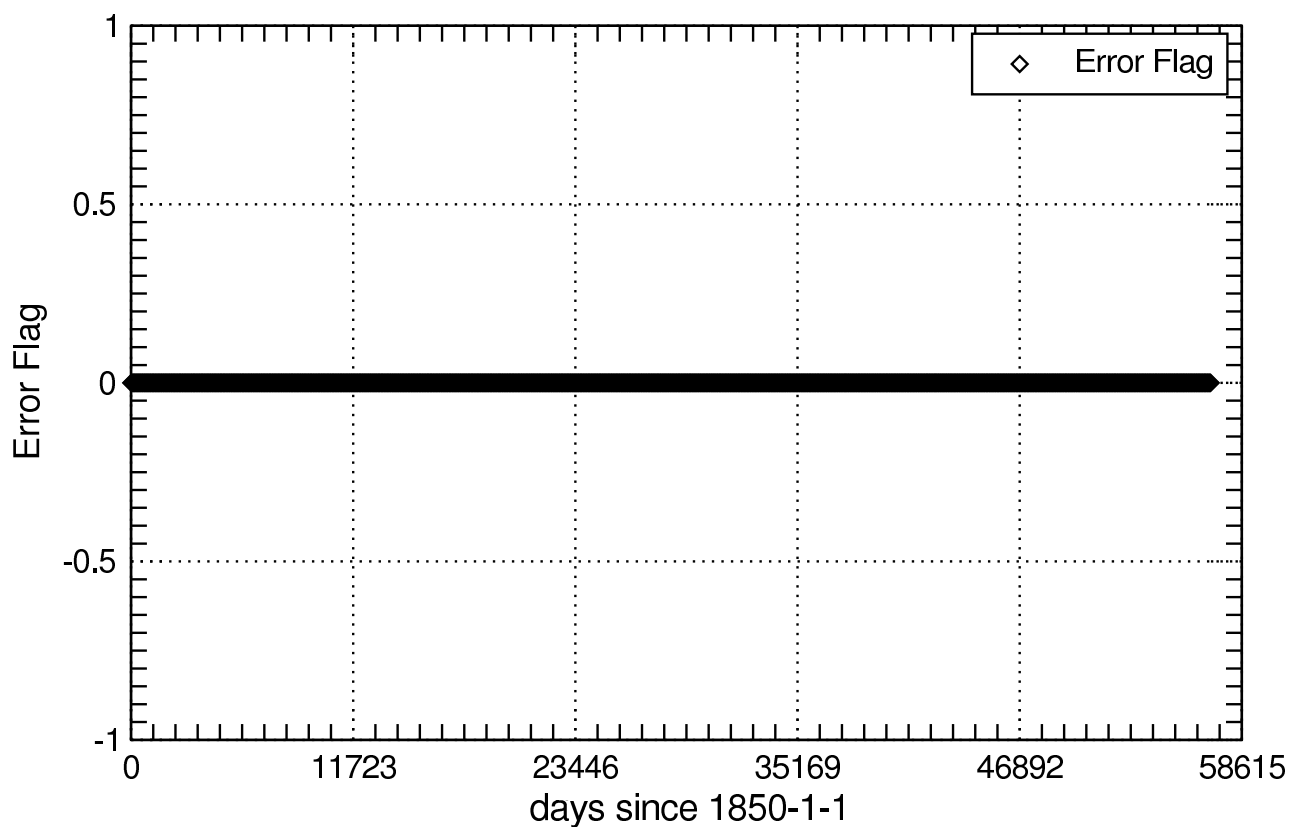
Error Flag of co2mass_Amon
