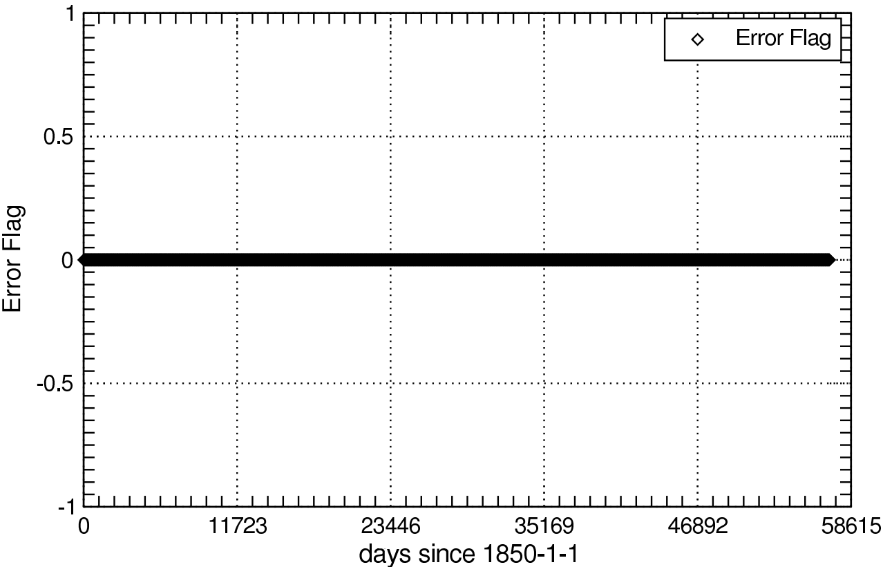
Error Flag of rlutcs_Amon
