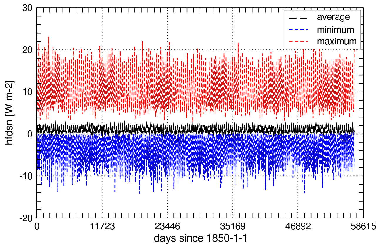
Global Values of hfdsn_Llmon
