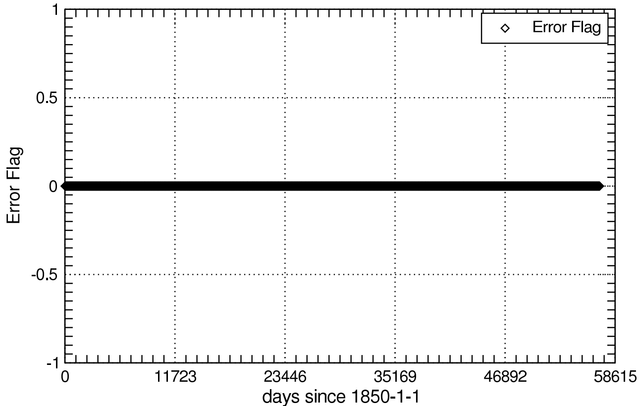
Error Flag of dryso4_aero
