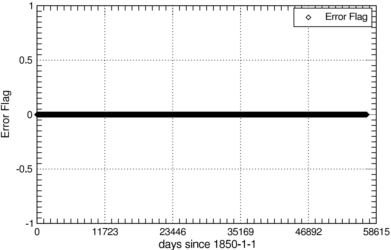
Error Flag of masscello_Omon
