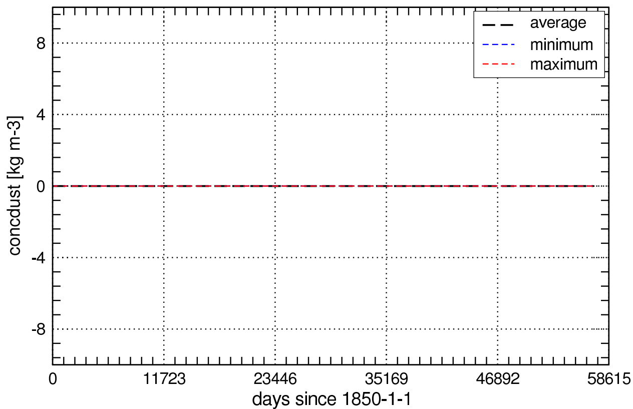
Global Values of concdust_aero
