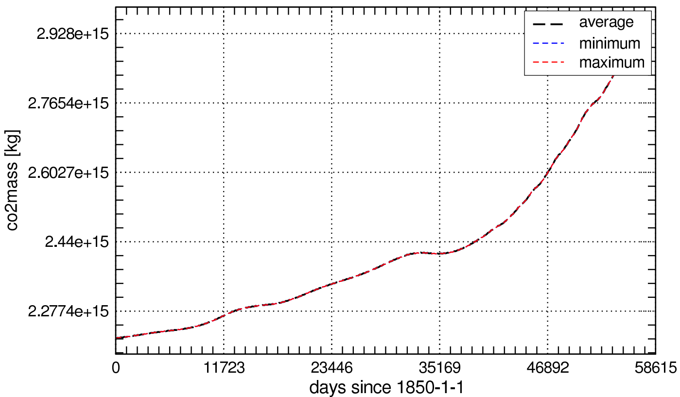
Global Values of co2mass_Amon
