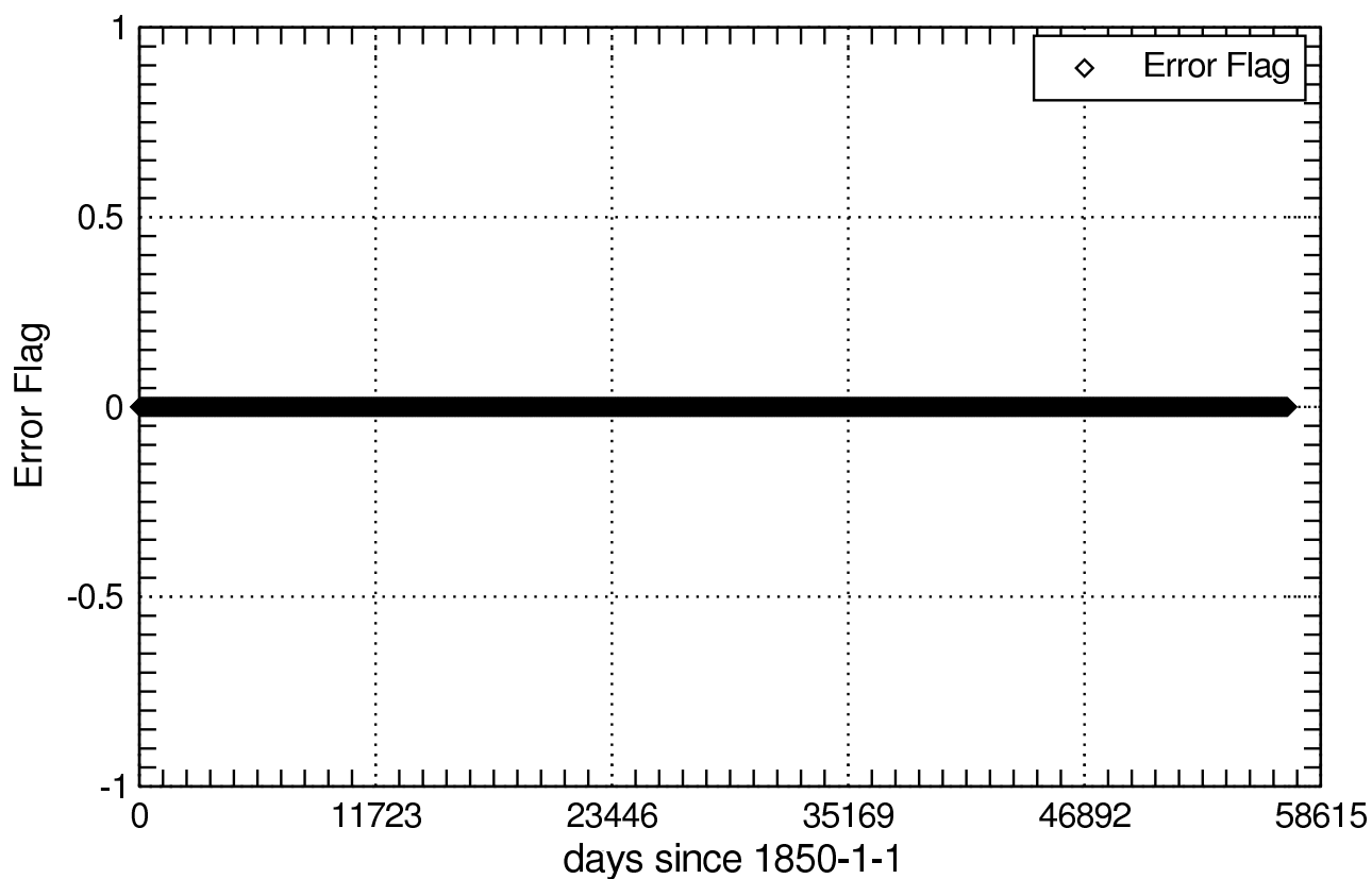
Error Flag of concdms_aero
