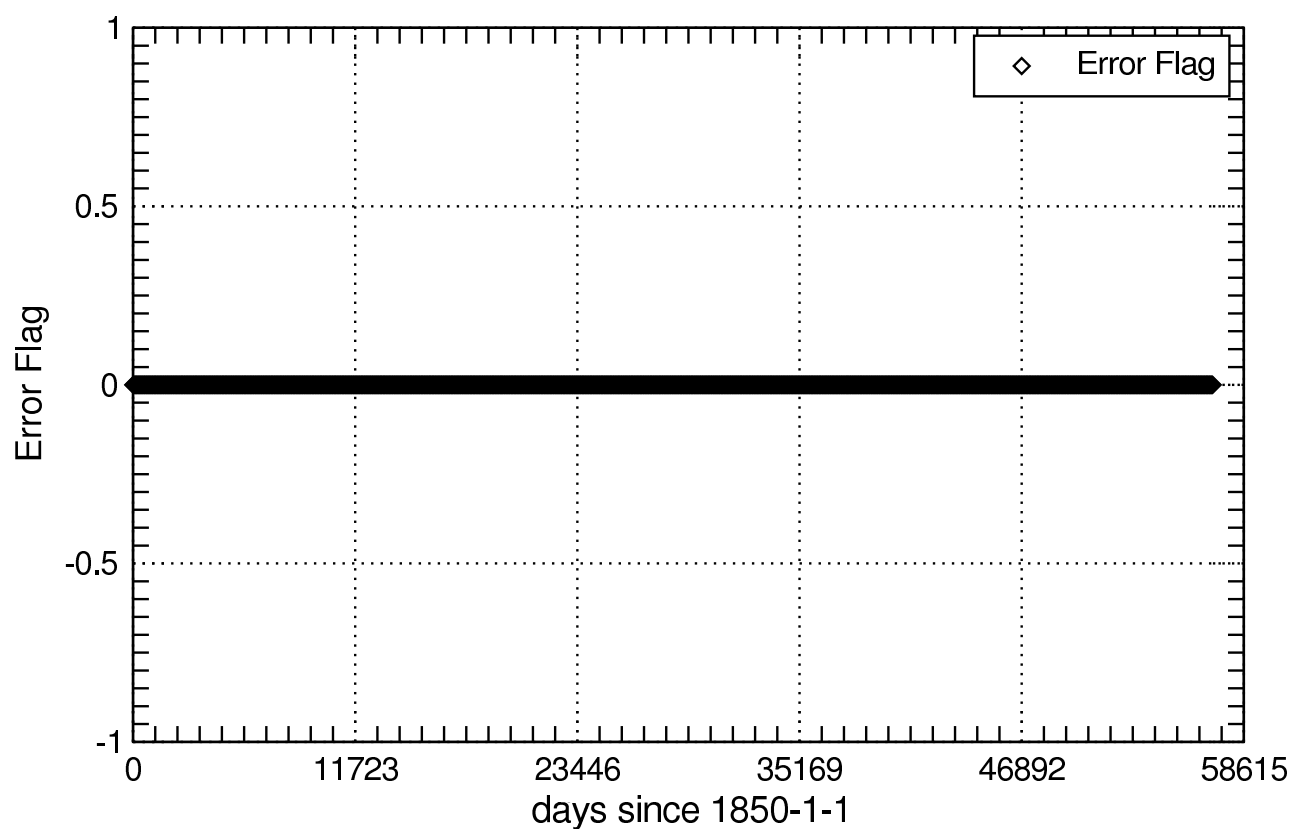
Error Flag of hfdsn_Llmon
