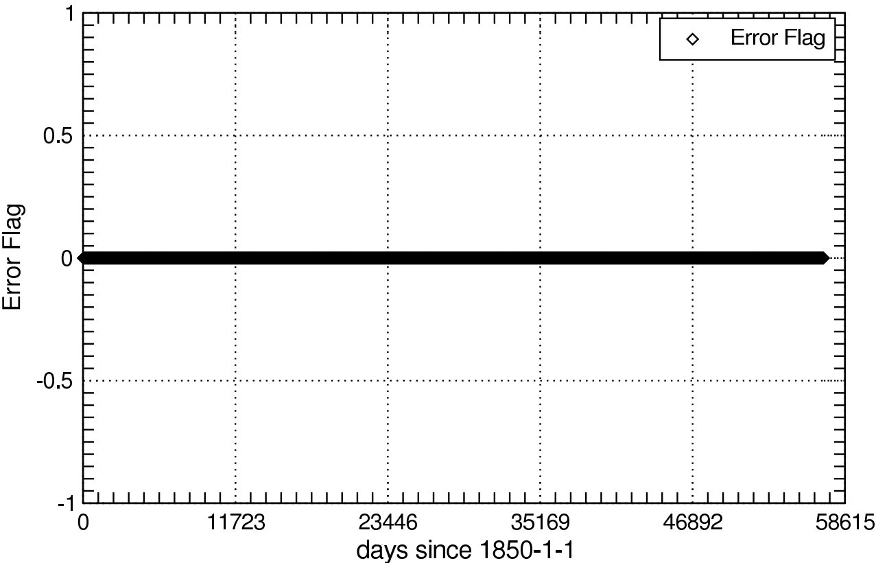
Error Flag of mrfso_Lmon
