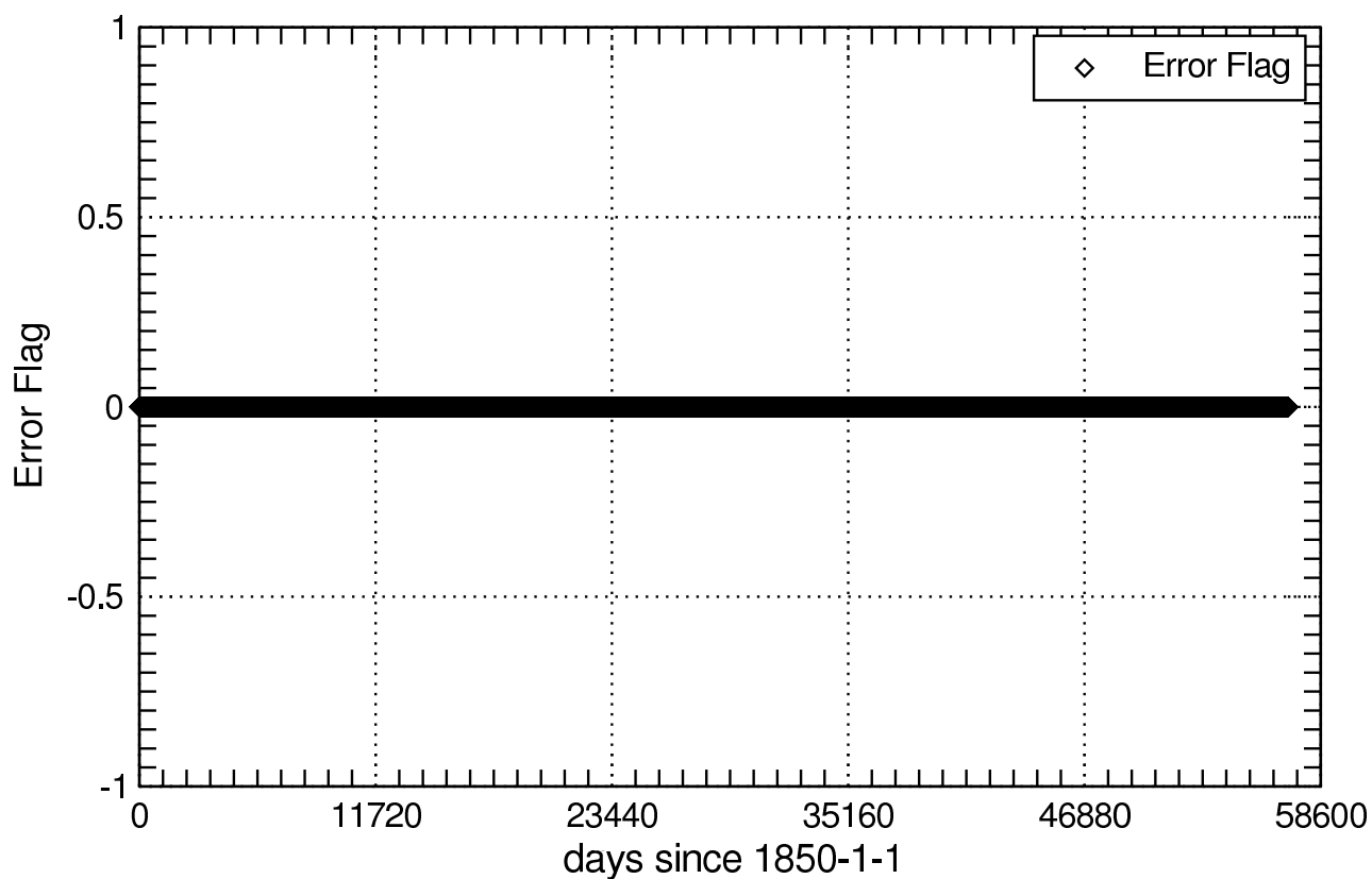
Error Flag of tasmin_day
