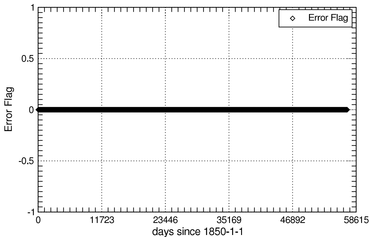
Error Flag of evspblveg_Lmon
