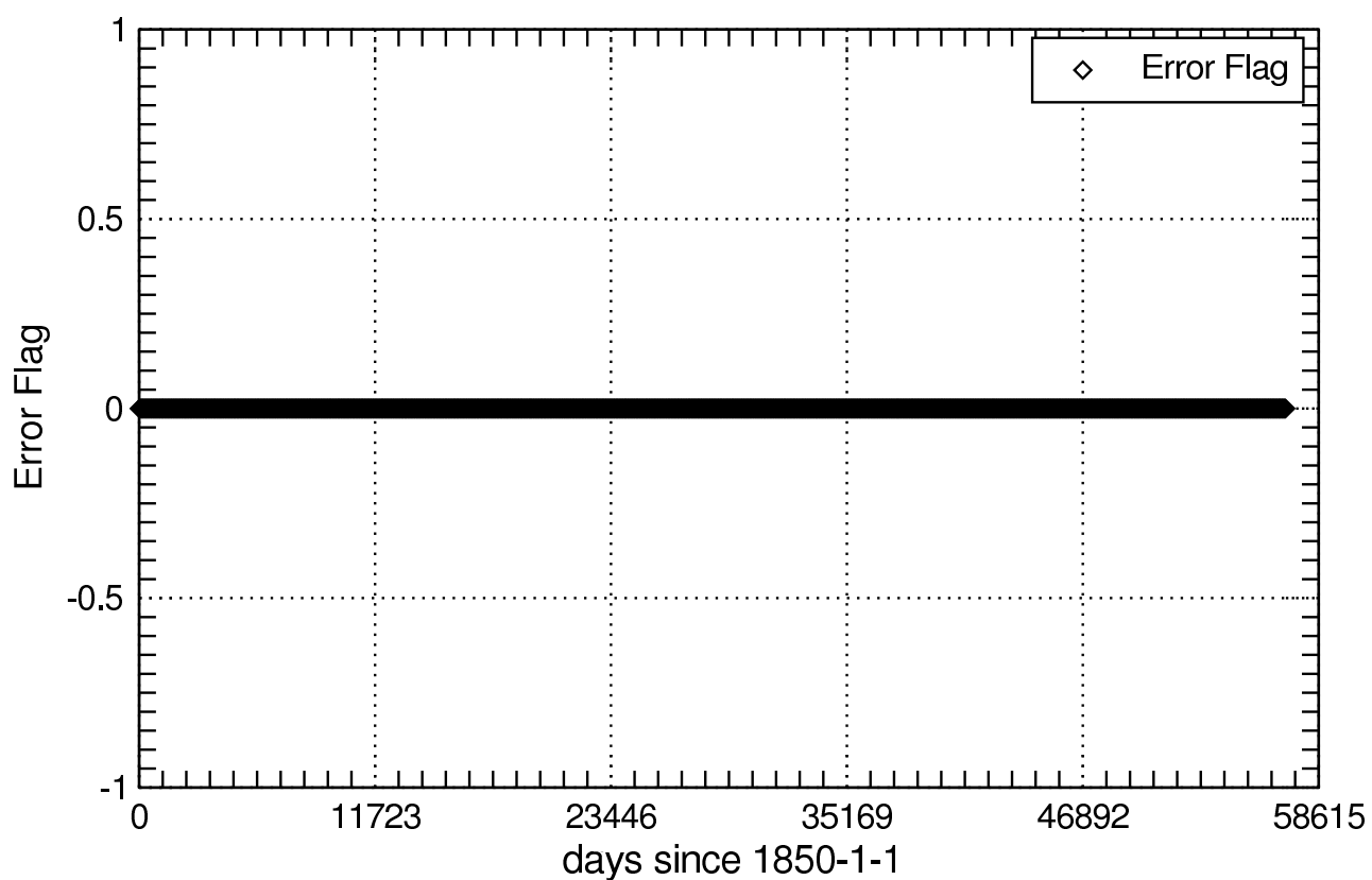
Error Flag of sconcdust_aero
