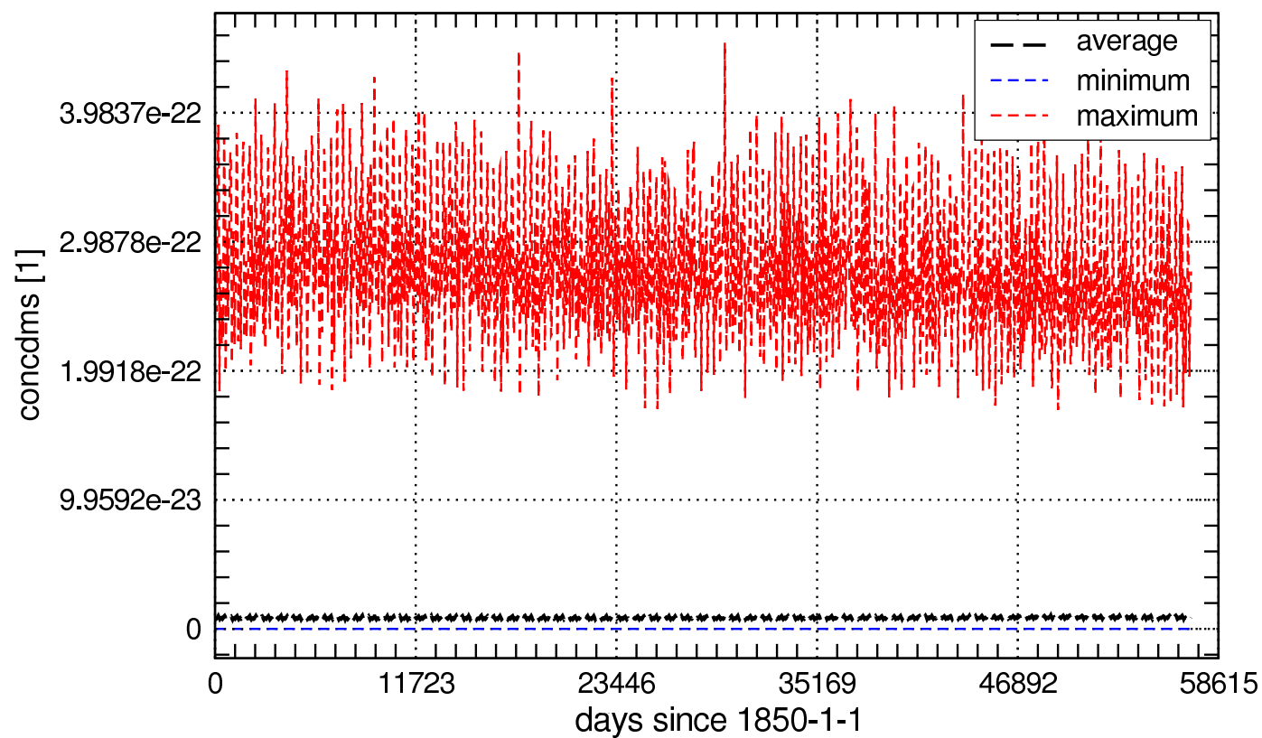
Global Values of concdms_aero
