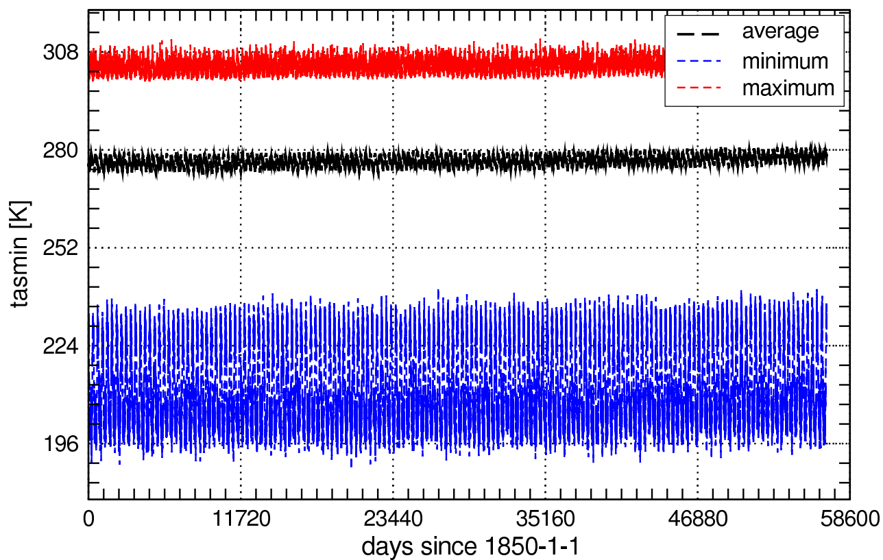
Global Values of tasmin_day
