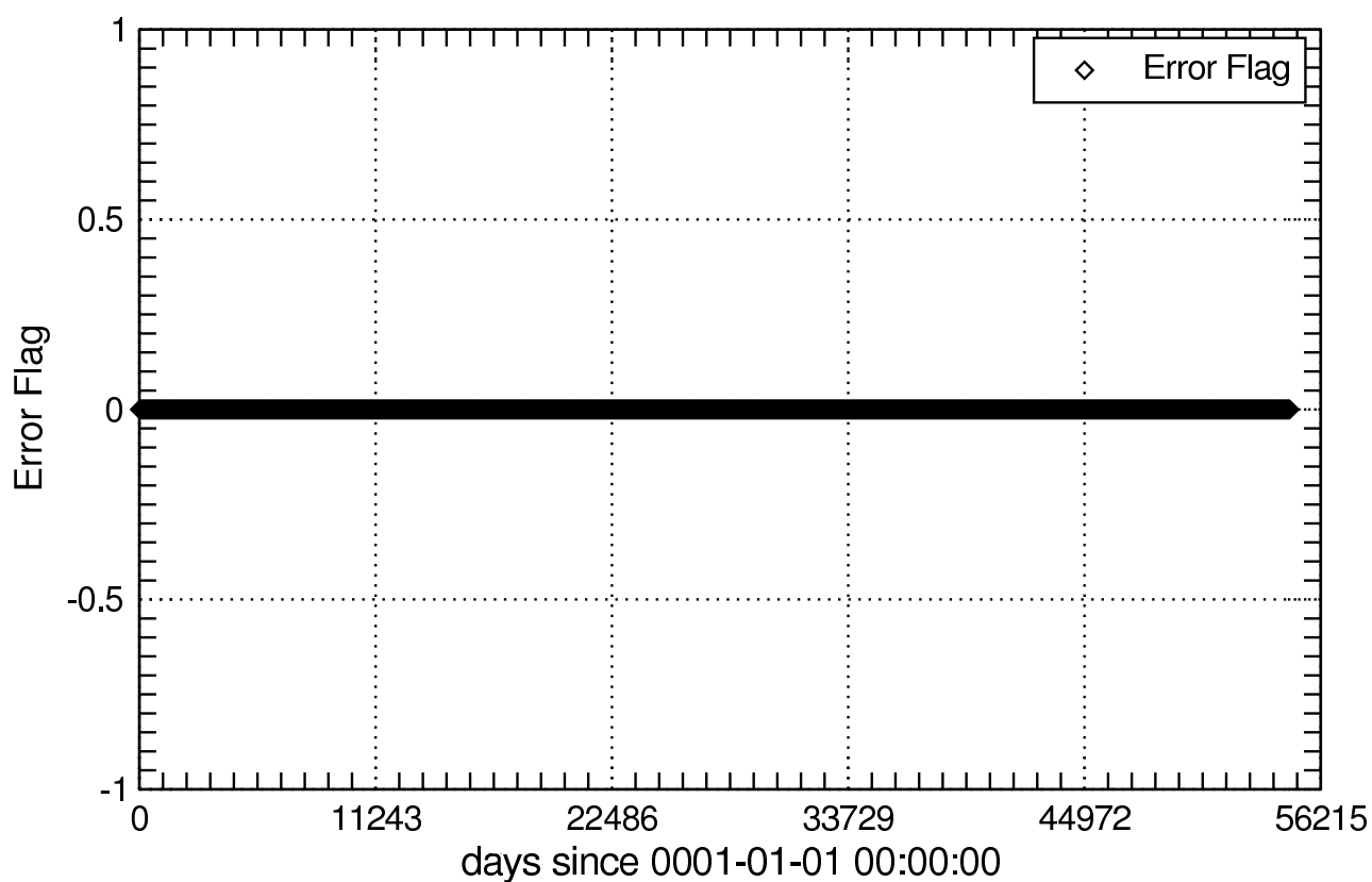
Error Flag of tasmin_Amon
