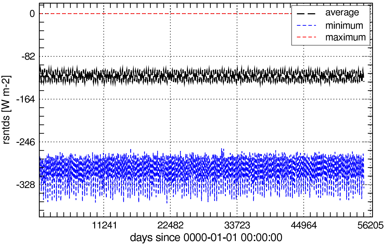
Global Values of rsntds_Omon
