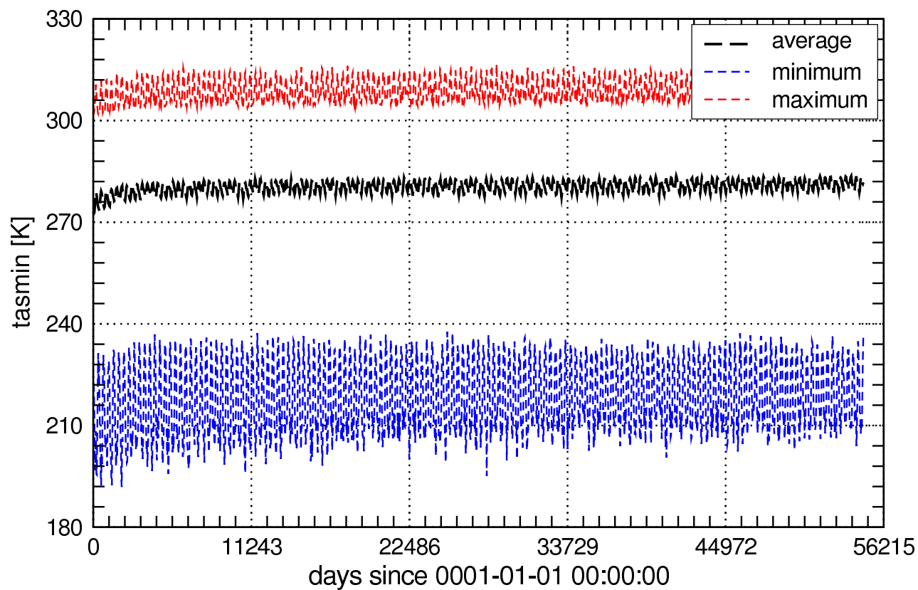
Global Values of tasmin_Amon
