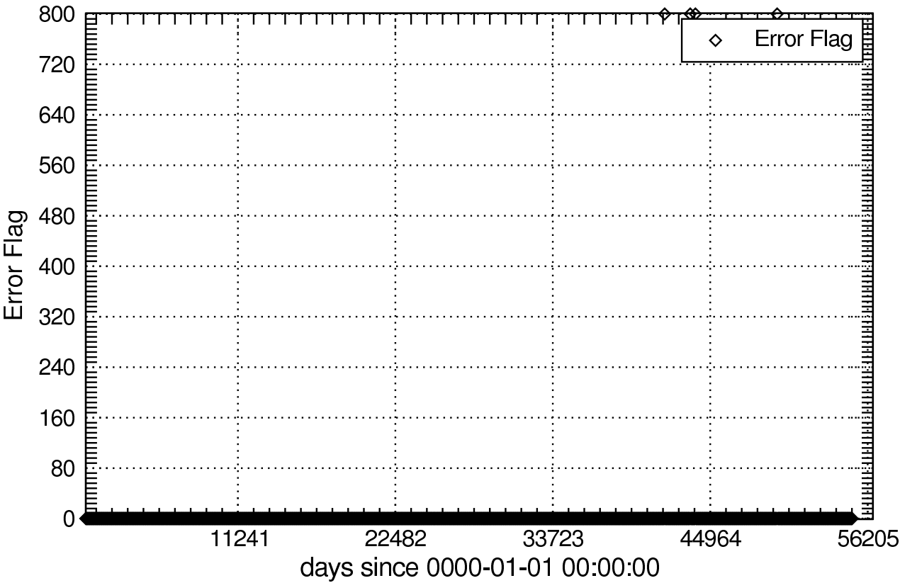
Error Flag of rsntds_Omon
