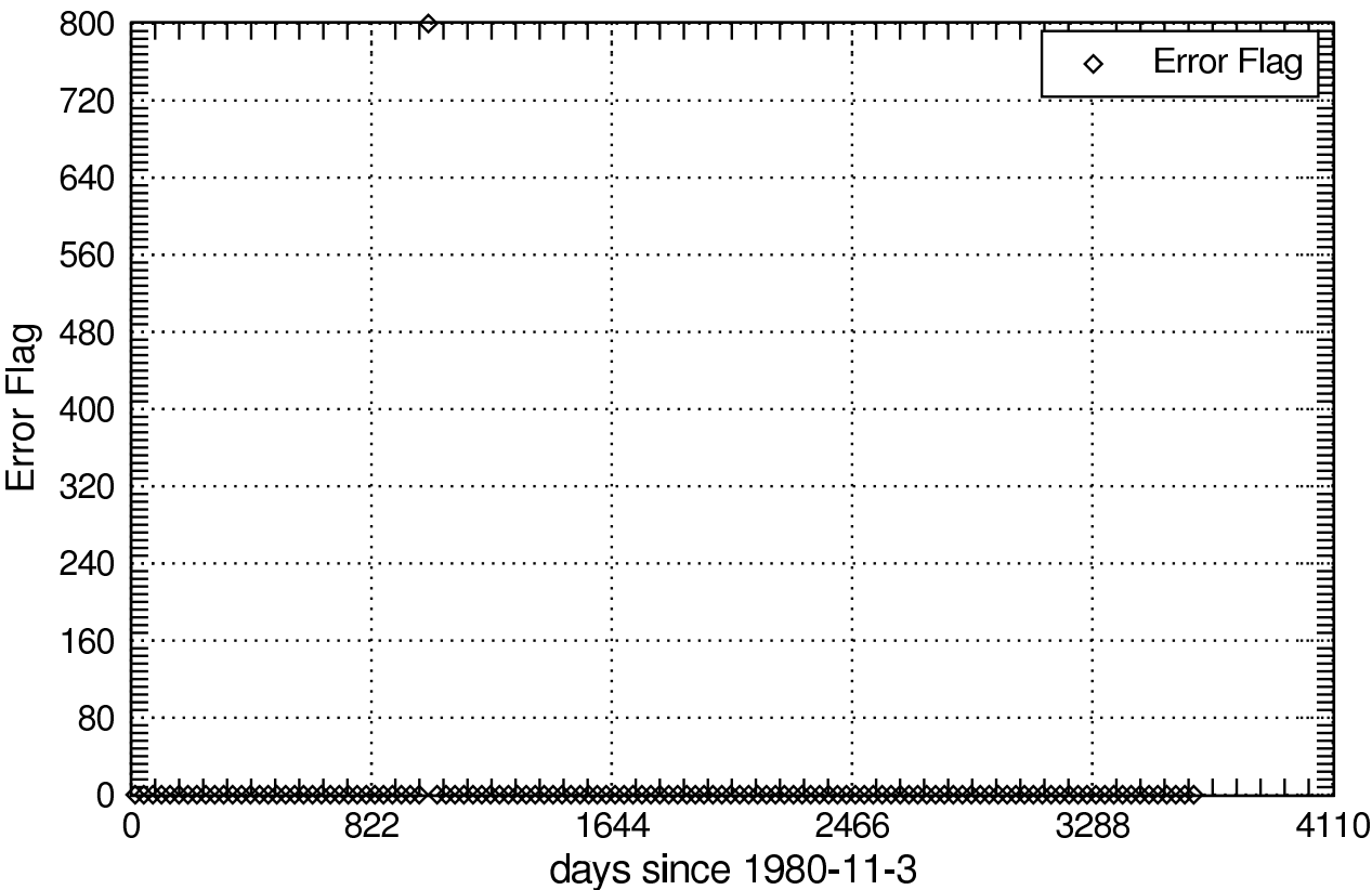
Error Flag of evpsblveg_Lmon
