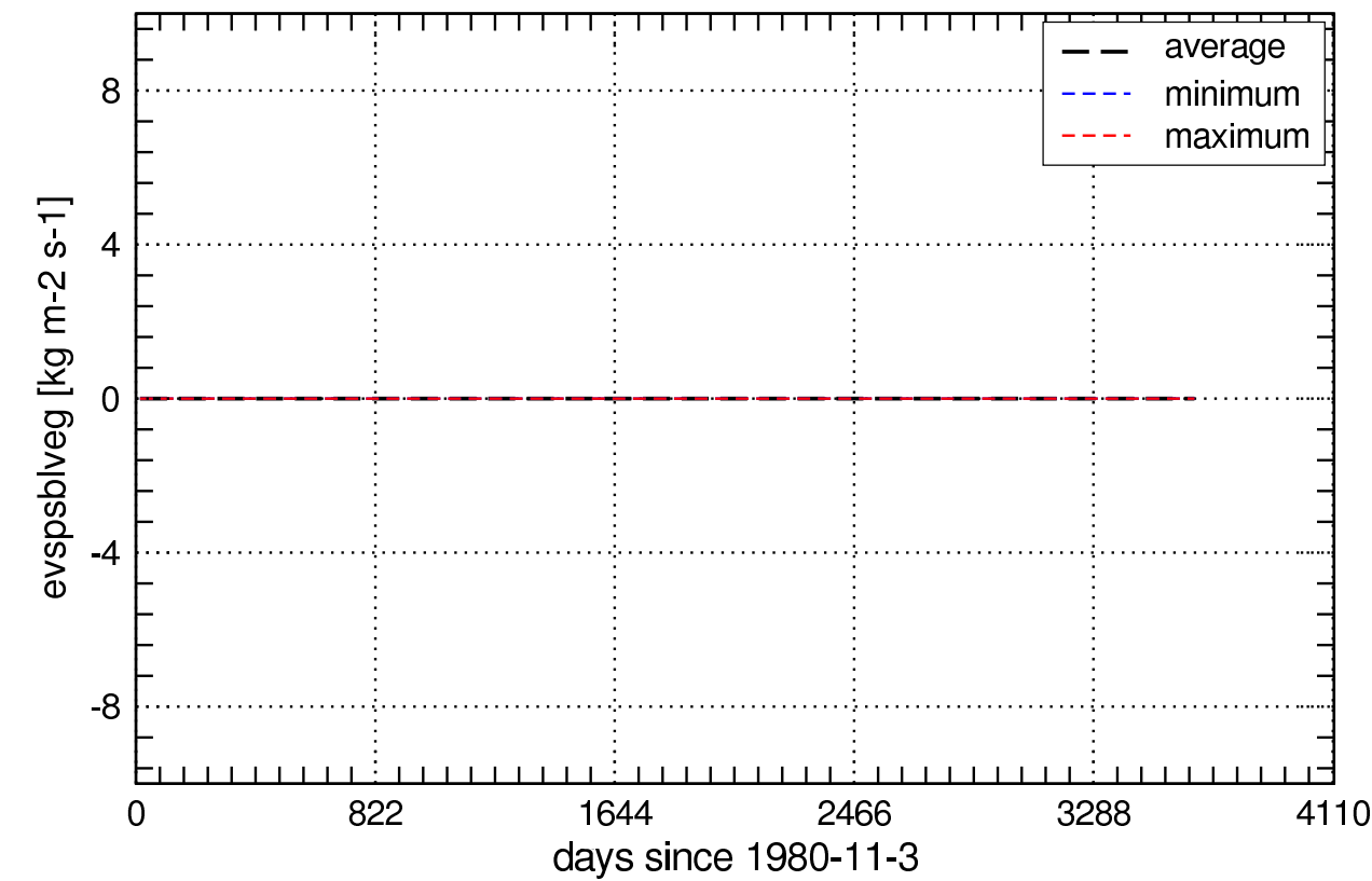
Global Values of evpsblveg_Lmon
