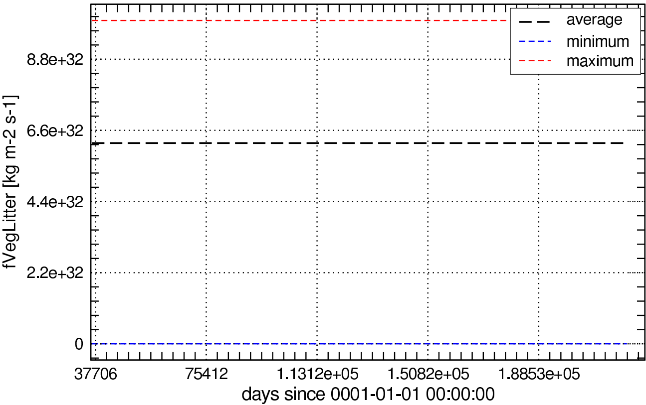
Global Values of fVegLitter_Lmon
